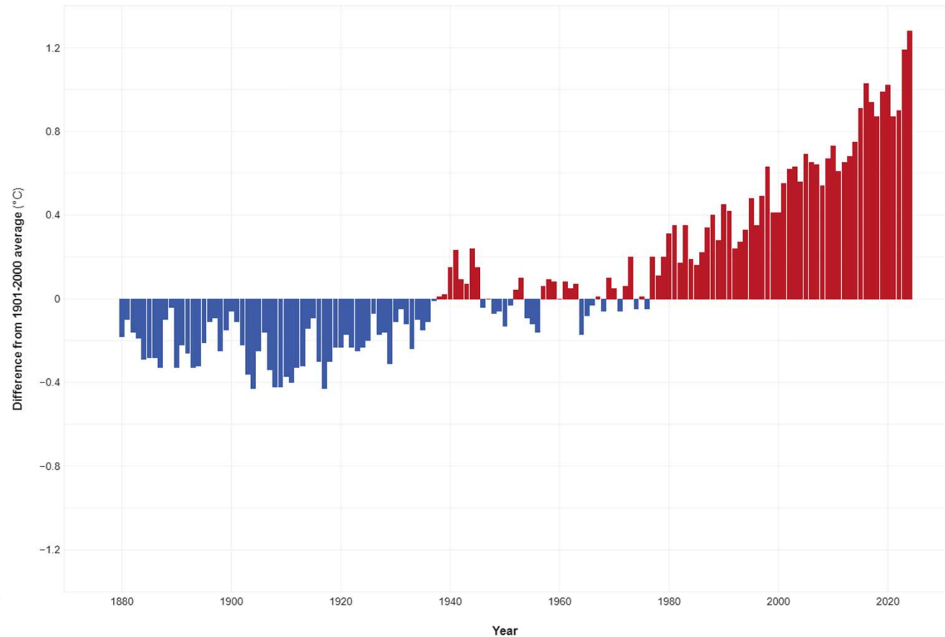
GLOBAL AVERAGE SURFACE TEMPERATURE
